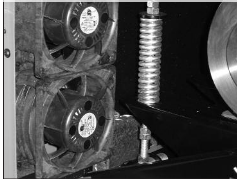
Roots patented automatic V-belt drive tensioning system and powerful cross-ventilation system for superior cooling.
